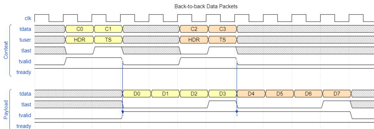
Figure 14: Two back-to-back packets on the AXIS Payload Context port (with header prefetching; CHDR_W = 64)
